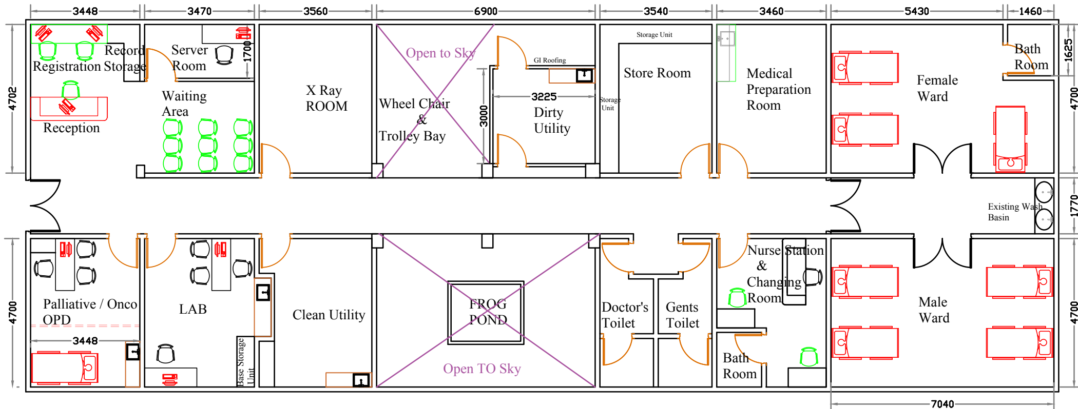
LAYOUT PLAN FOR THE PROPOSED ACCF DAY CARE CHEMOWARD AND OPD AT F.A.A.M.C.H. BARPETA.
